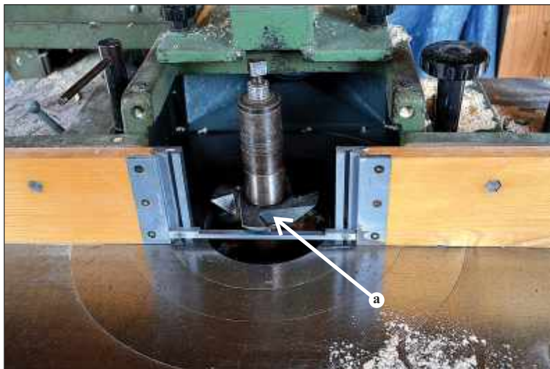
Frezarka – Kc, Nd; fot. JK a – frez – Kc
